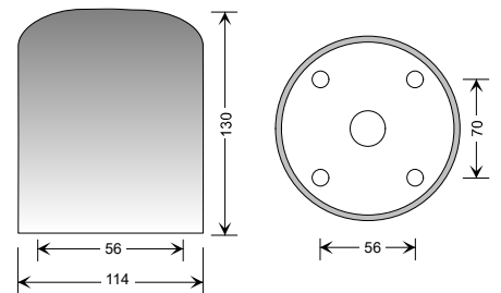
DIMENSIONS TYPE 3 WEIGHT 6,2Kg
